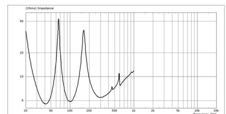
LS400 impedance
